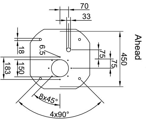
Deck Drilling Scheme
