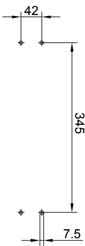
Drilling Scheme
